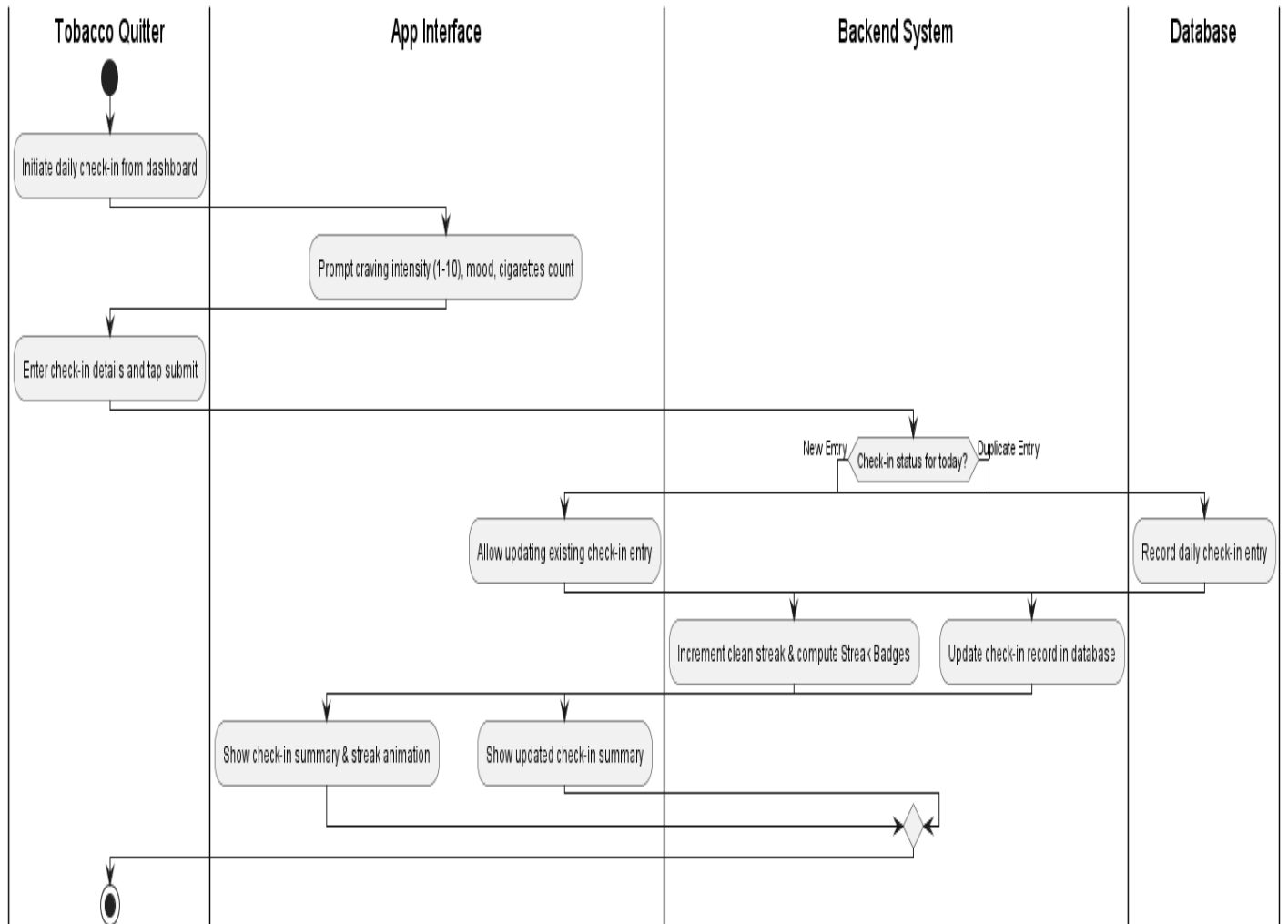
Figure 25: Swimlane Diagram for Daily Check-in
