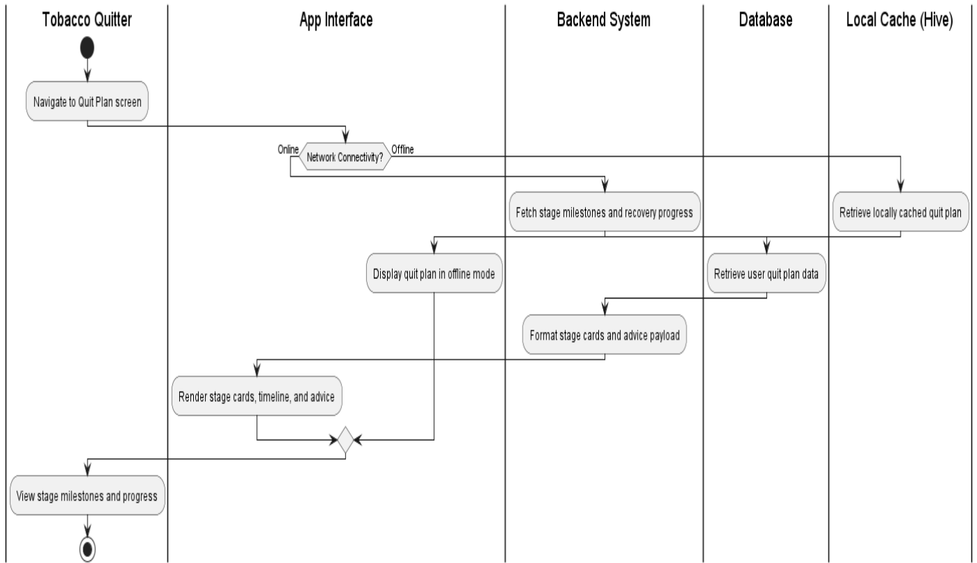
Figure 24: Swimlane Diagram for View Quit Plan
