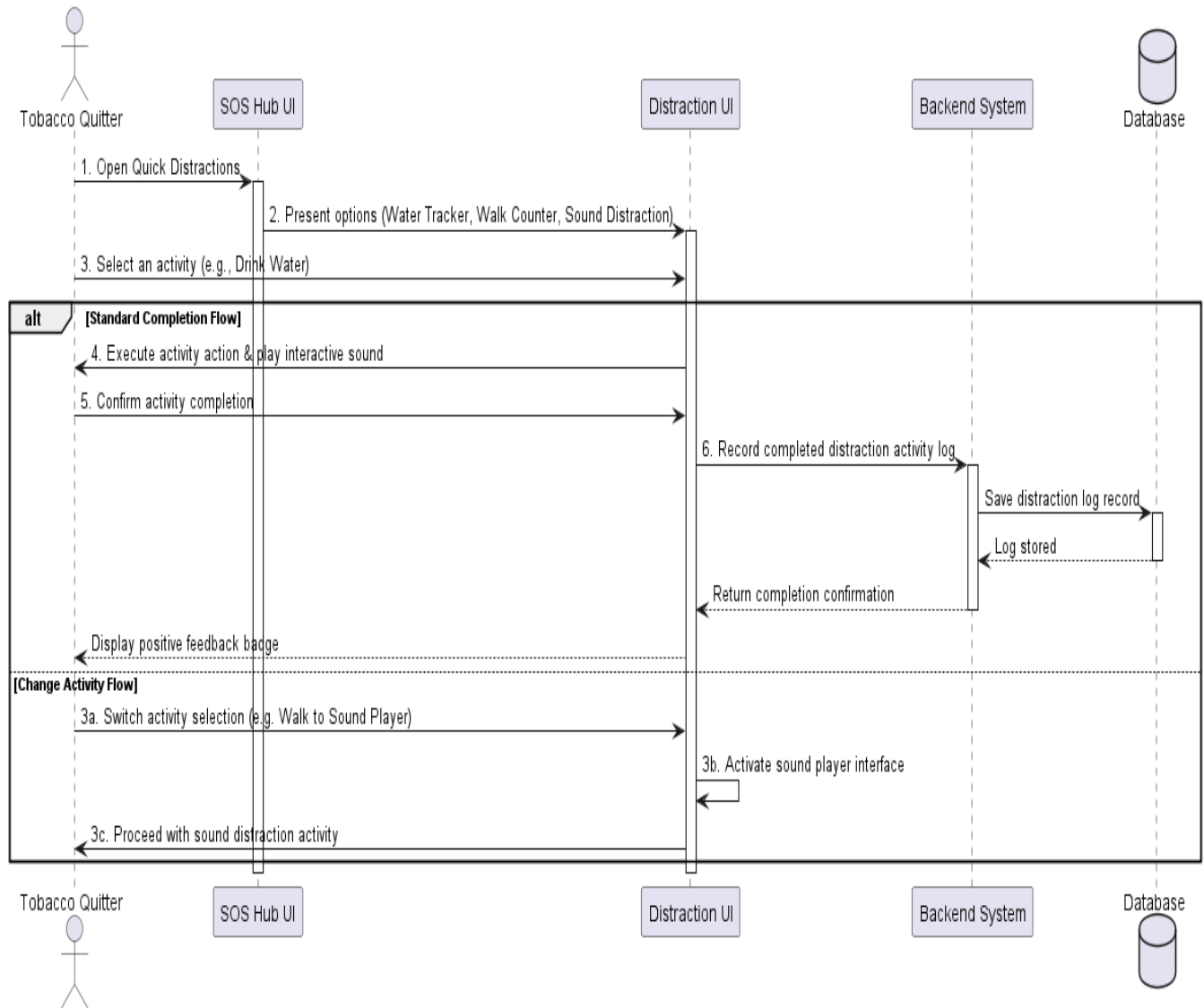
Figure 20: Sequence Diagram for Quick Distraction
