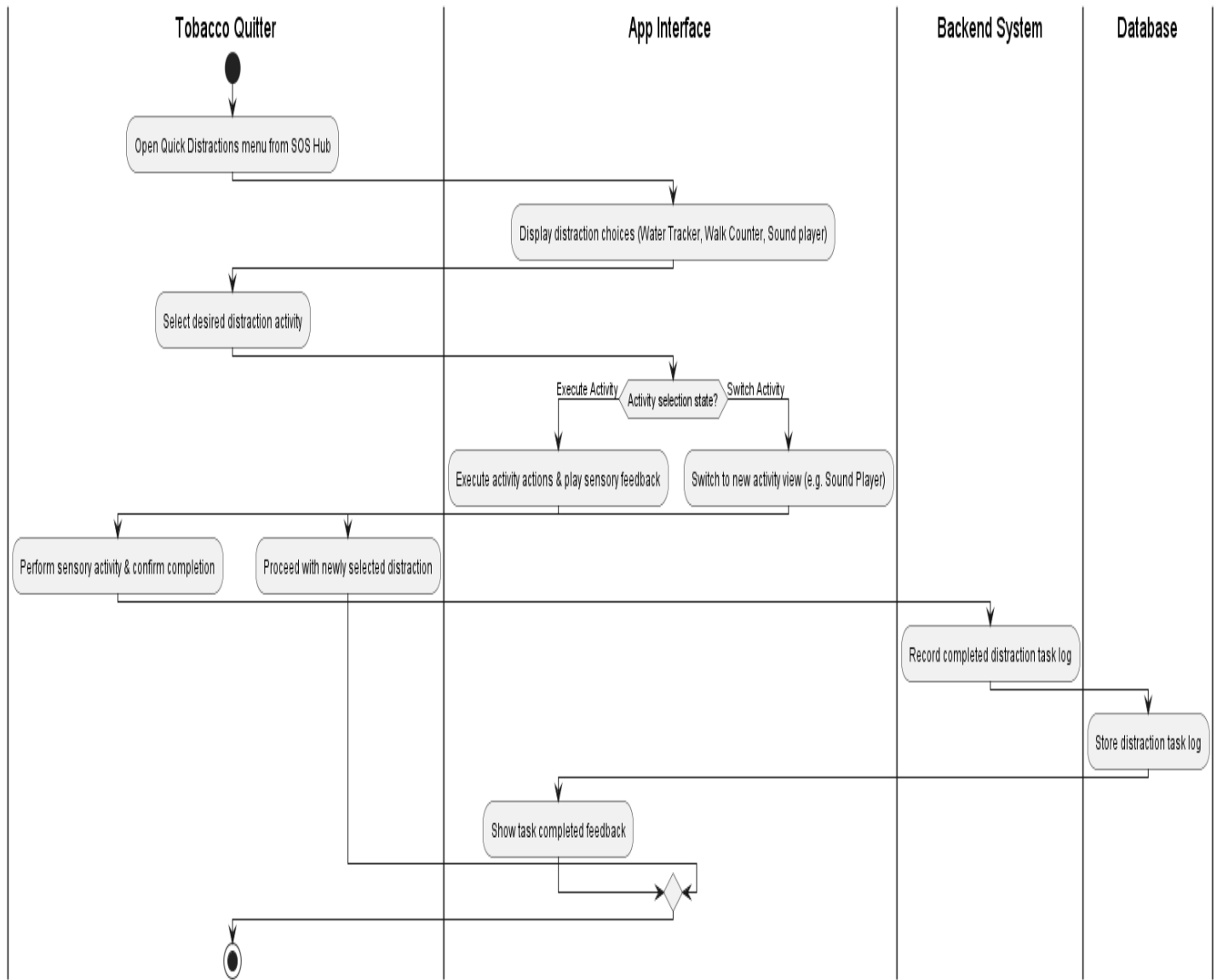
Figure 30: Swimlane Diagram for Quick Distraction
