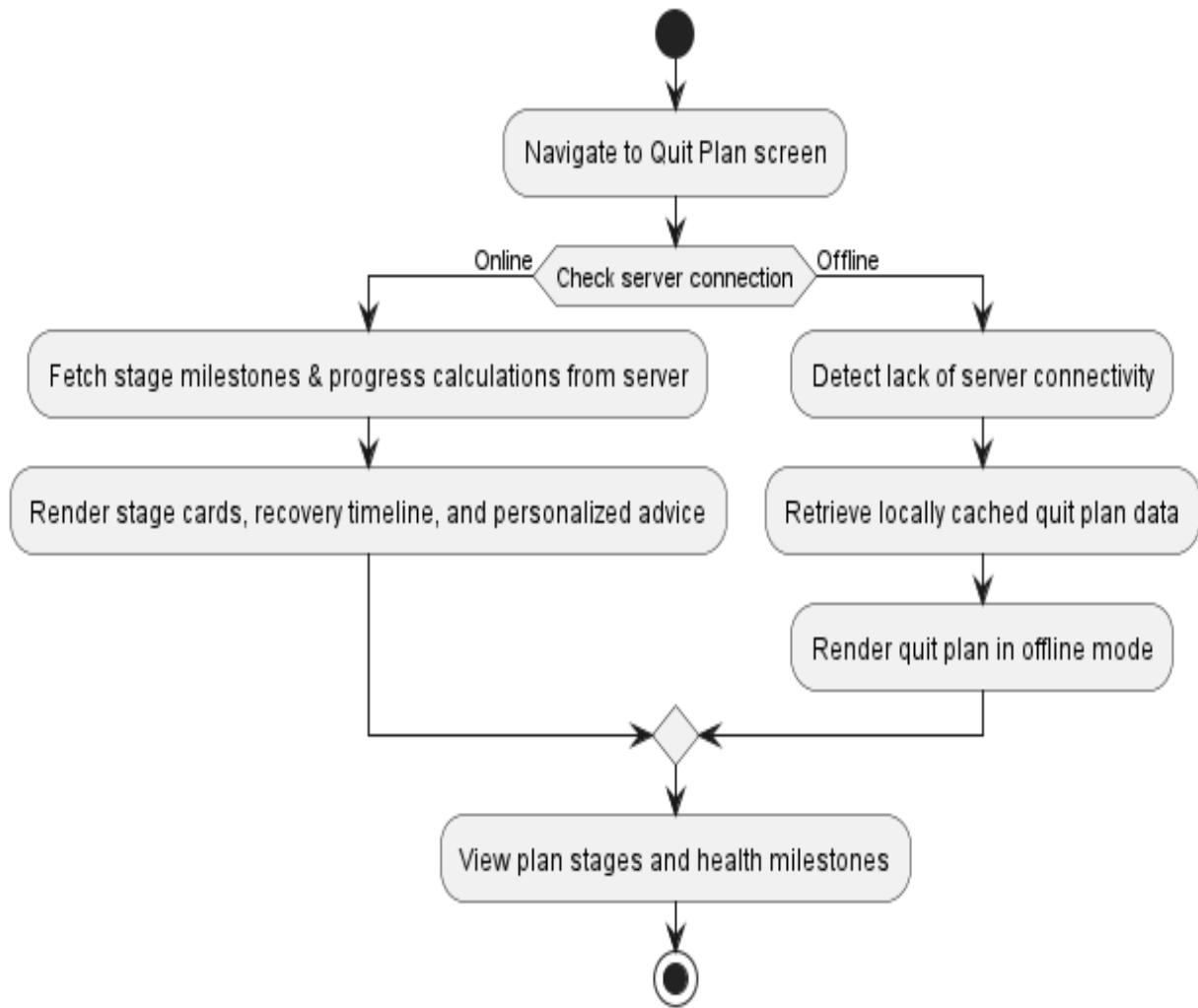
Figure 4: Activity Diagram for View Quit Plan
