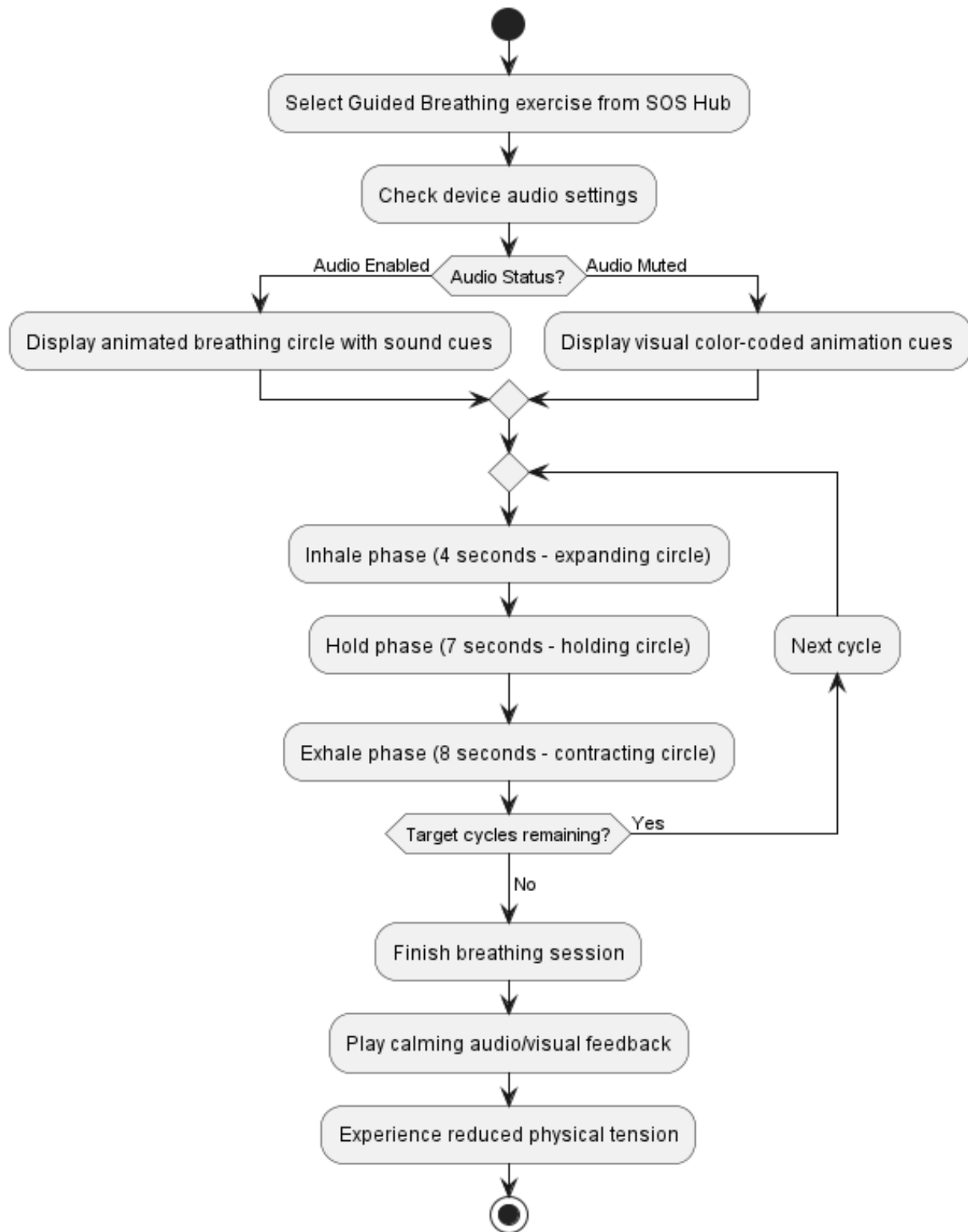
Figure 9: Activity Diagram for Breathing Exercise
