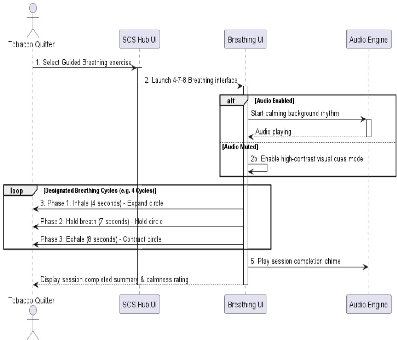
Figure 19: Sequence Diagram for Breathing Exercise
