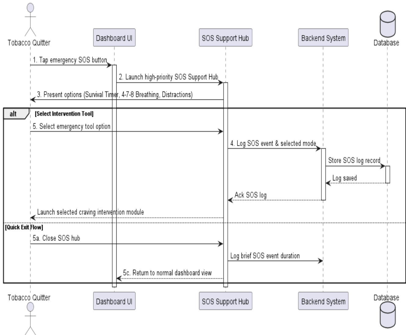
Figure 17: Sequence Diagram for Craving Support
