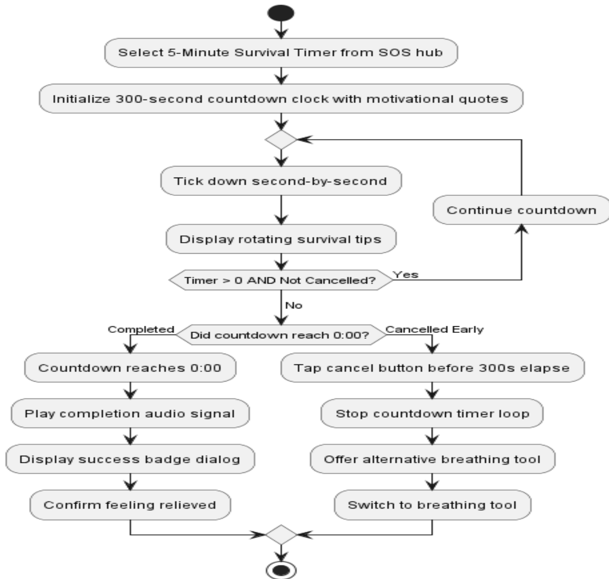
Figure 8: Activity Diagram for Start Survival Timer
