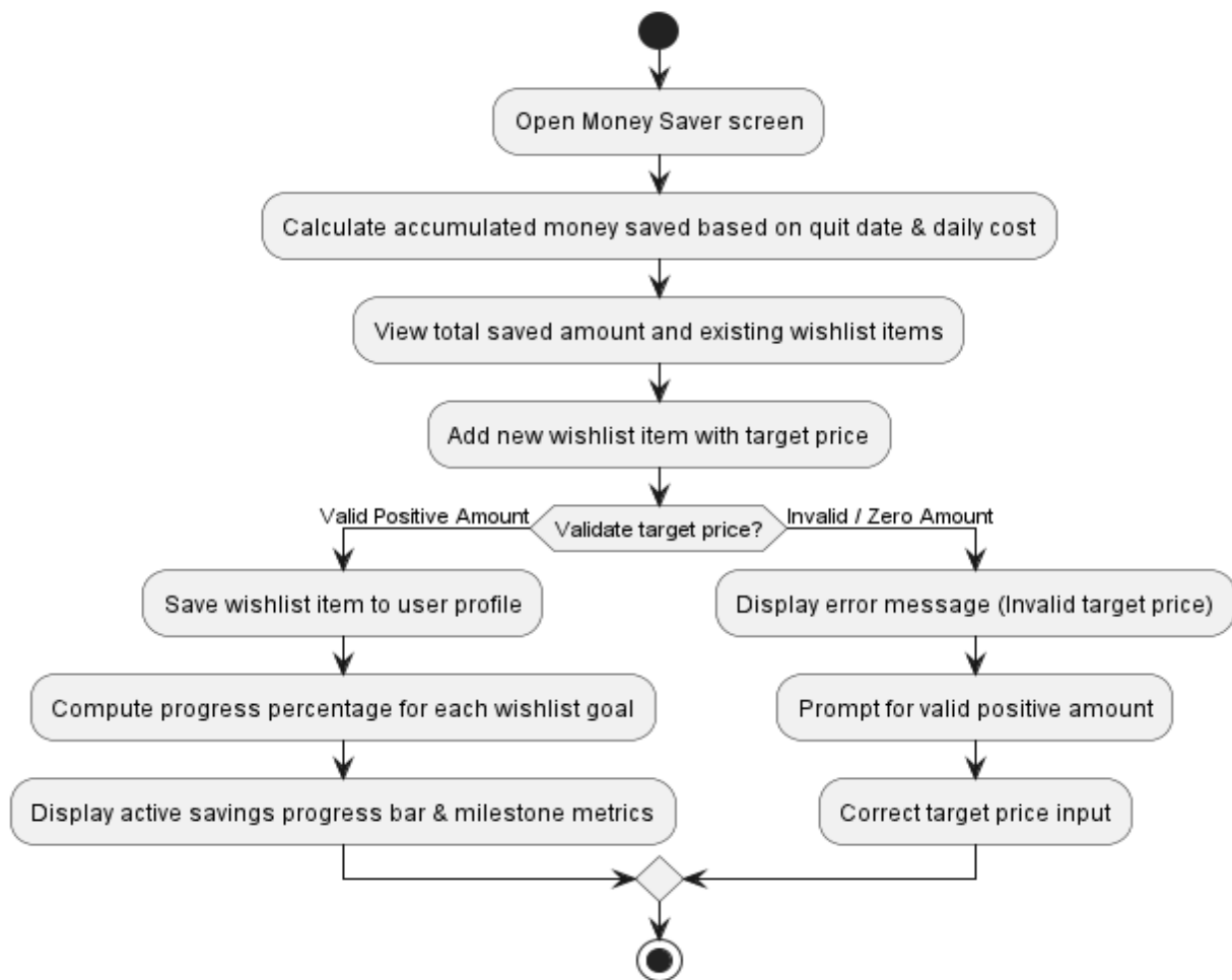
Figure 6: Activity Diagram for Track Saving
