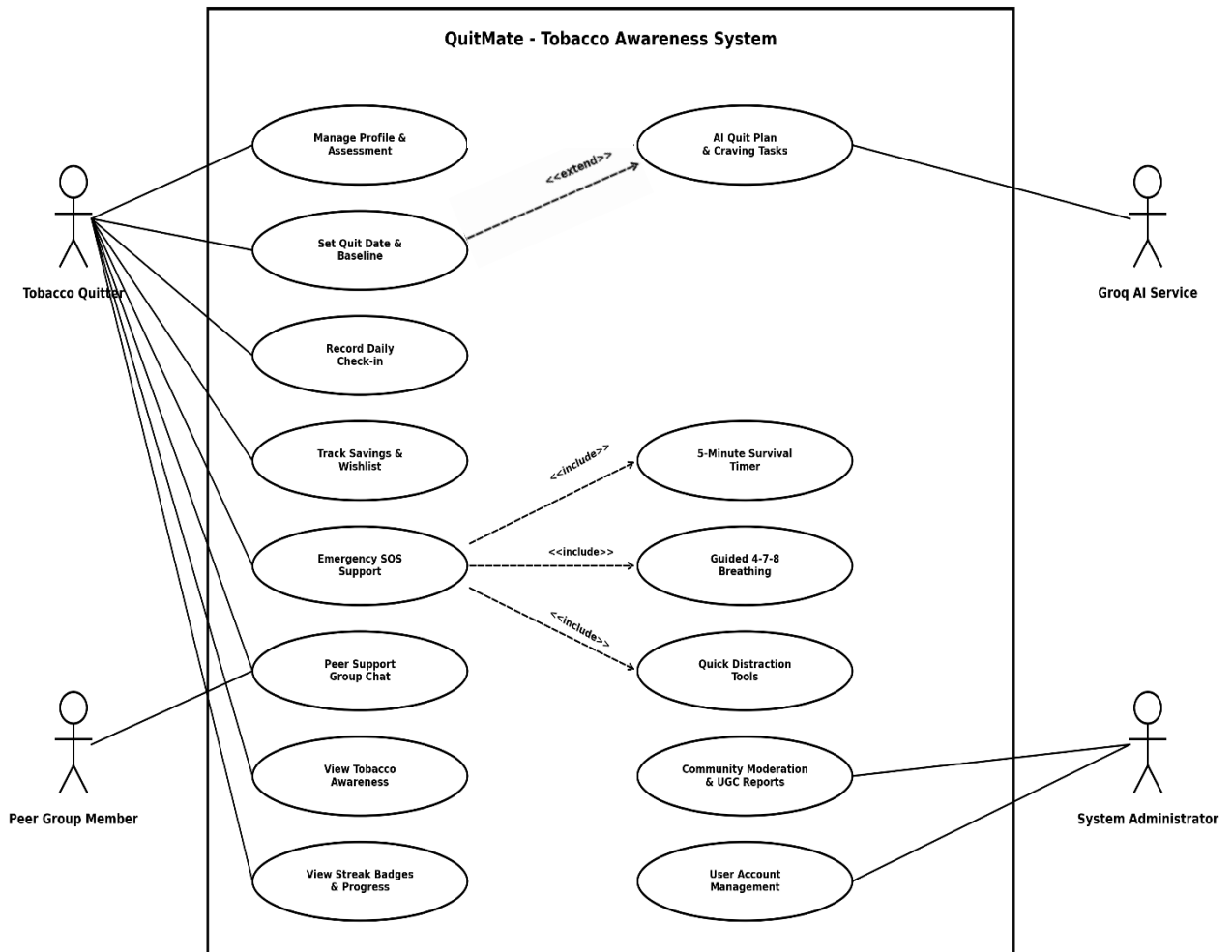
Figure 1: Use Case Diagram for QuitMate - Tobacco Awareness
