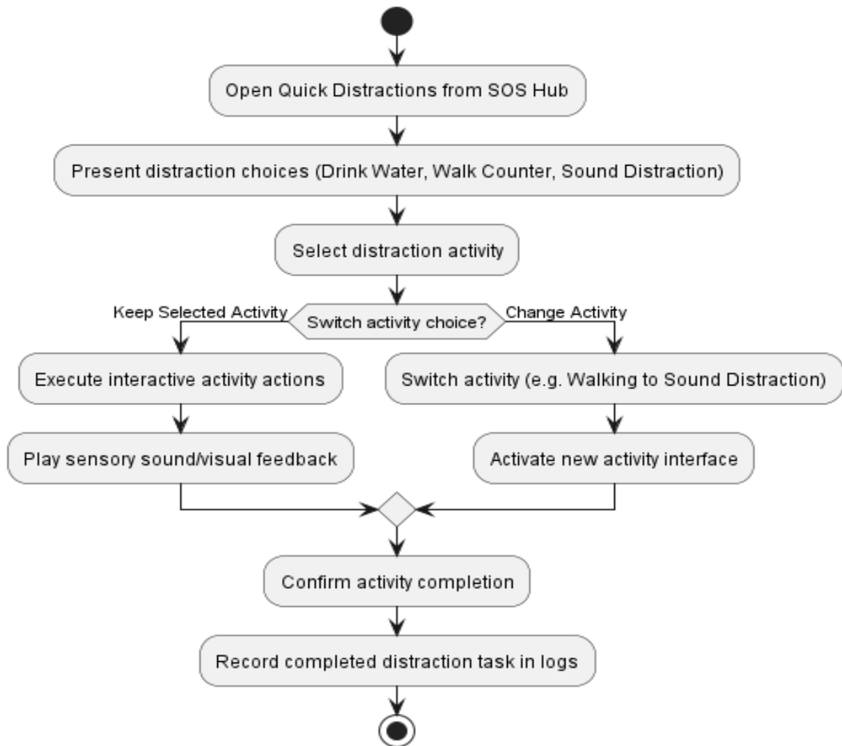
Figure 10: Activity Diagram for Quick Distraction
