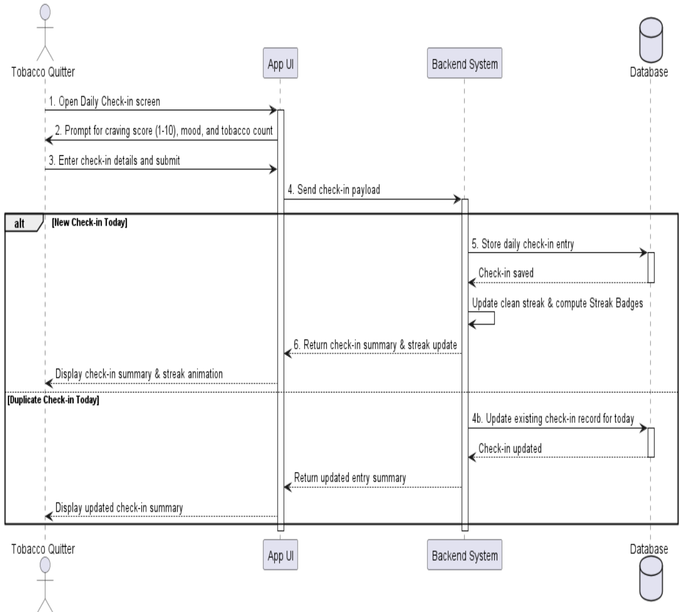
Figure 15: Sequence Diagram for Daily Check-in
