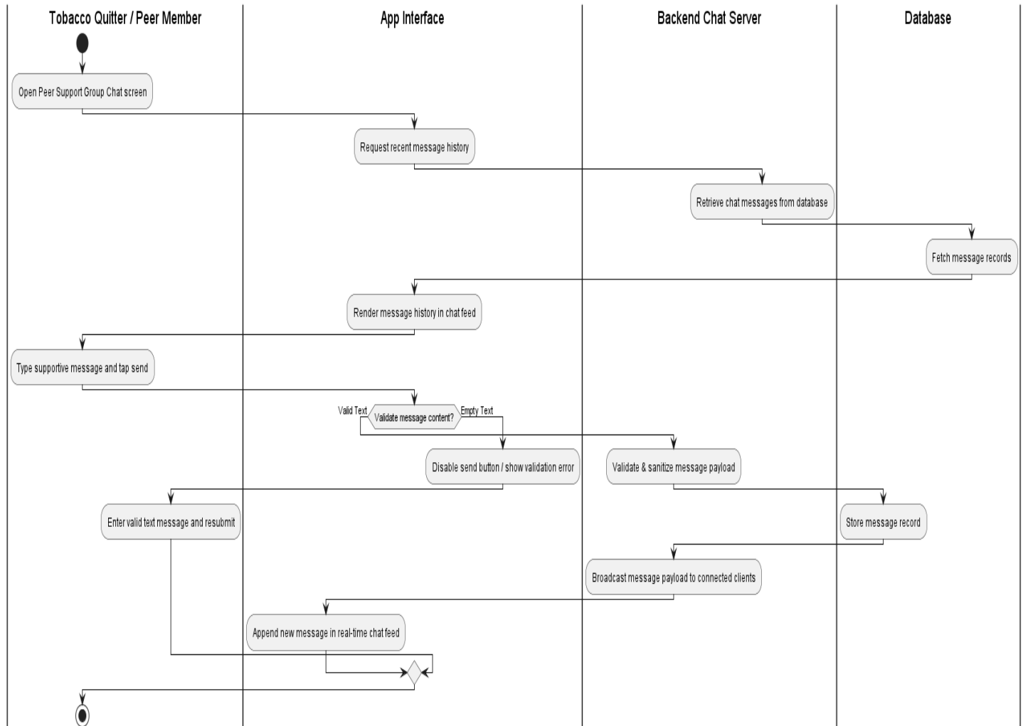
Figure 31: Swimlane Diagram for Access Peer Support Group
