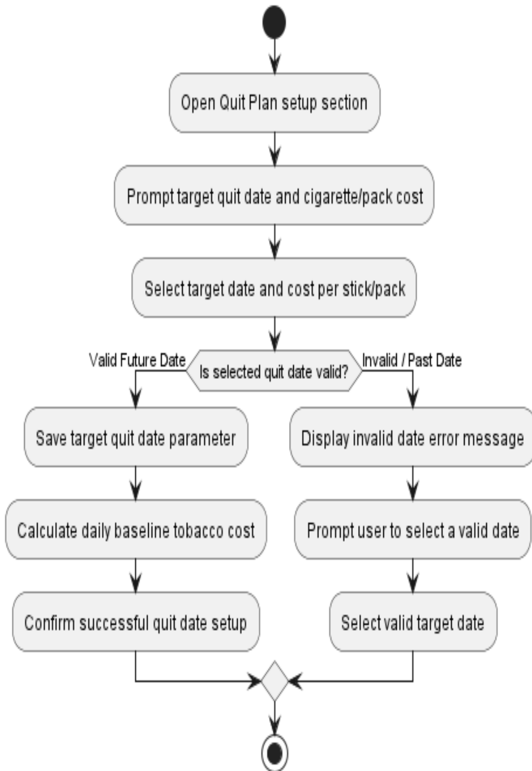
Figure 3: Activity Diagram for Set Quit Date
