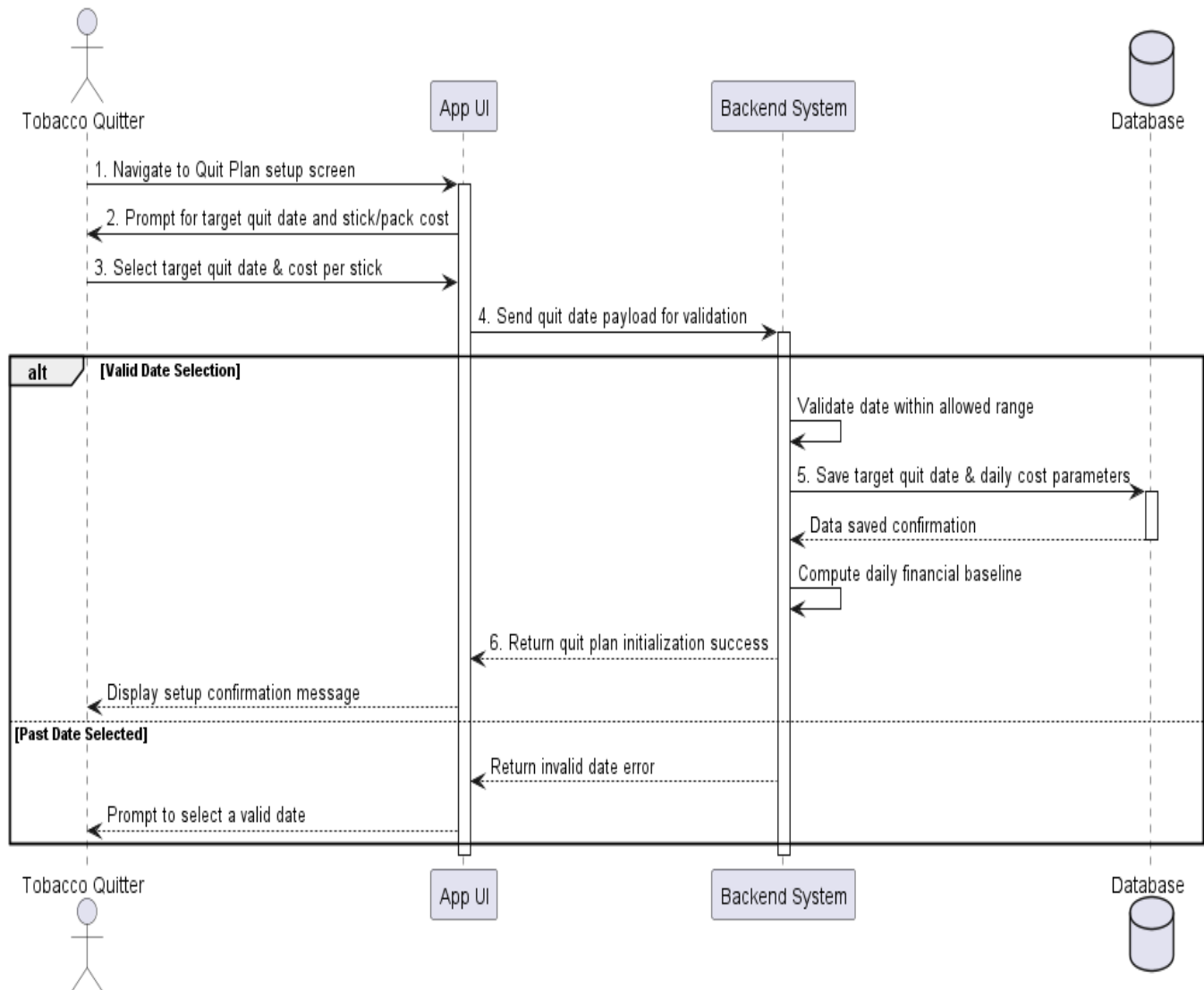
Figure 13: Sequence Diagram for Set Quit Date
