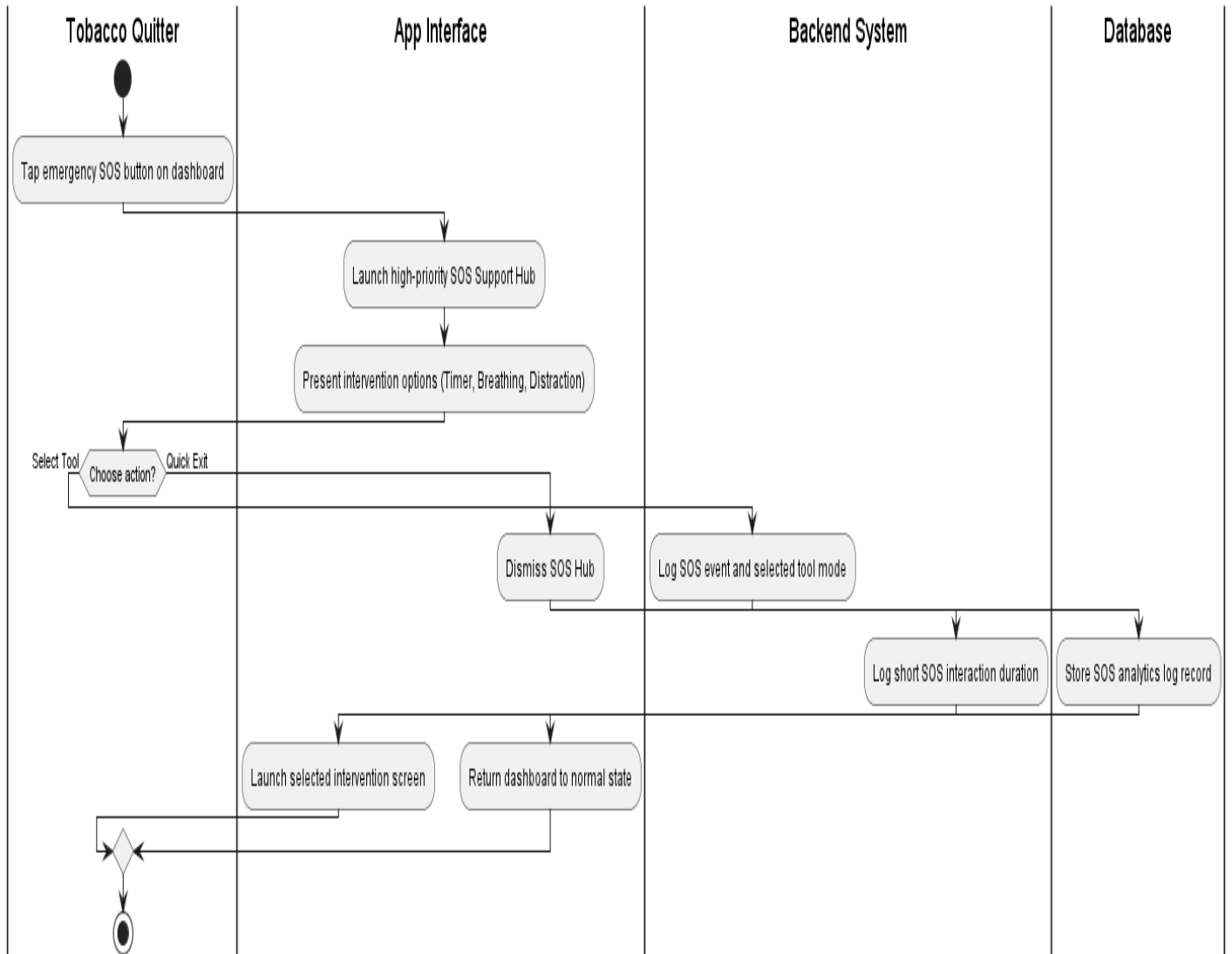
Figure 27: Swimlane Diagram for Craving Support
