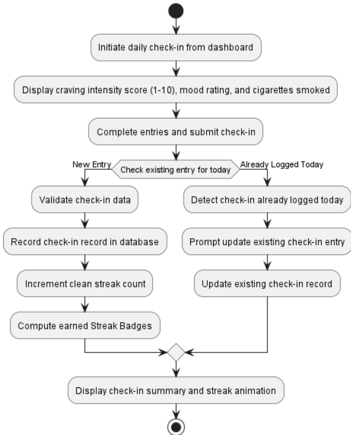
Figure 5: Activity Diagram for Daily Check-in
