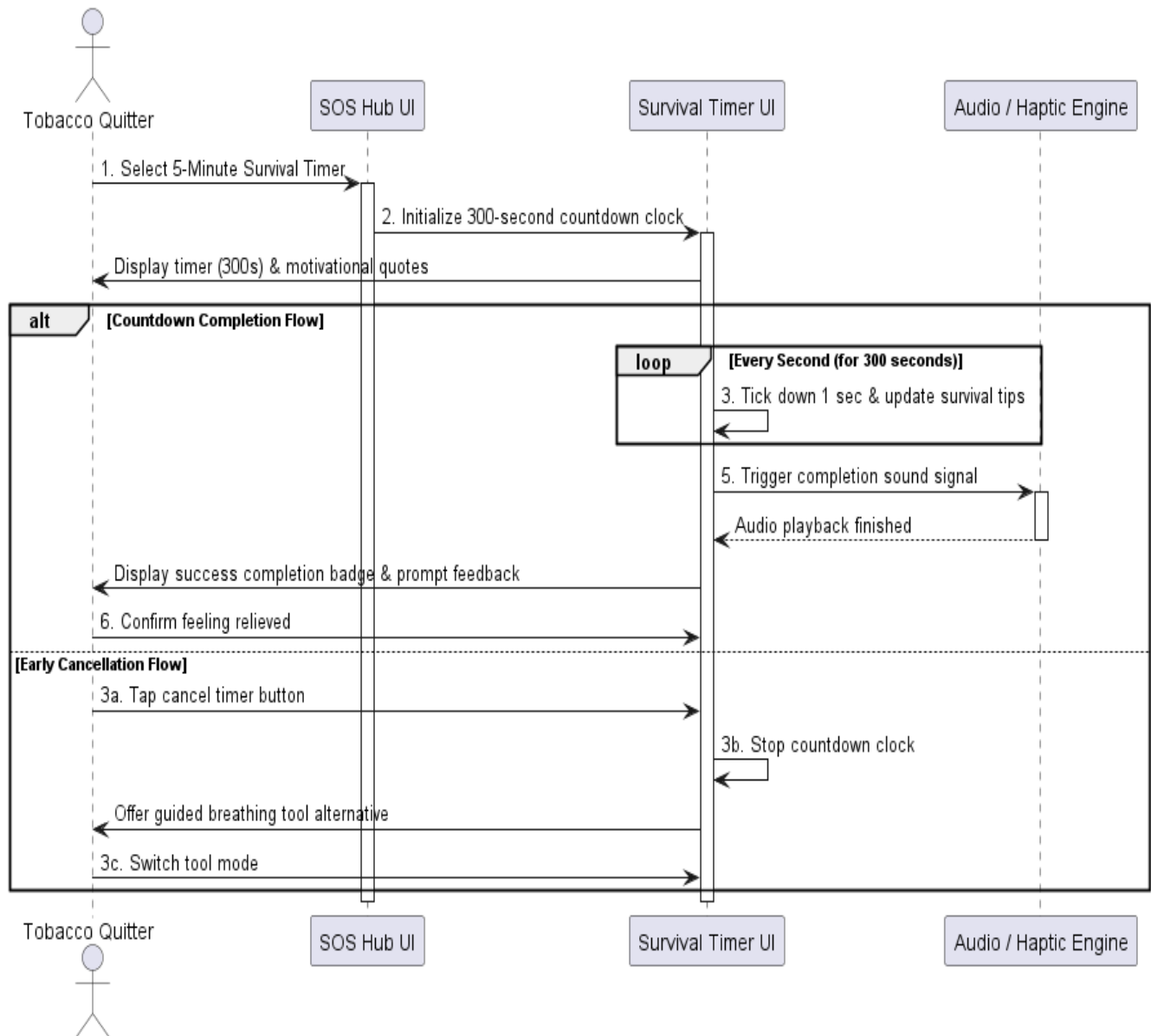
Figure 18: Sequence Diagram for Start Survival Timer
