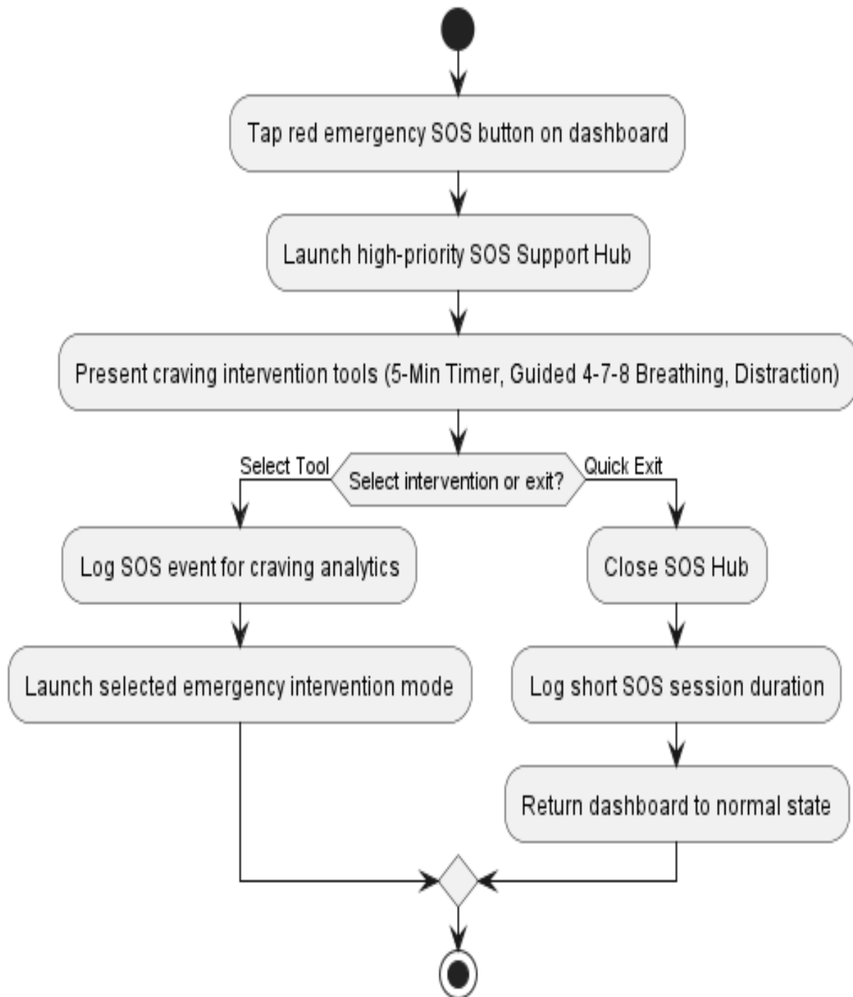
Figure 7: Activity Diagram for Craving Support
