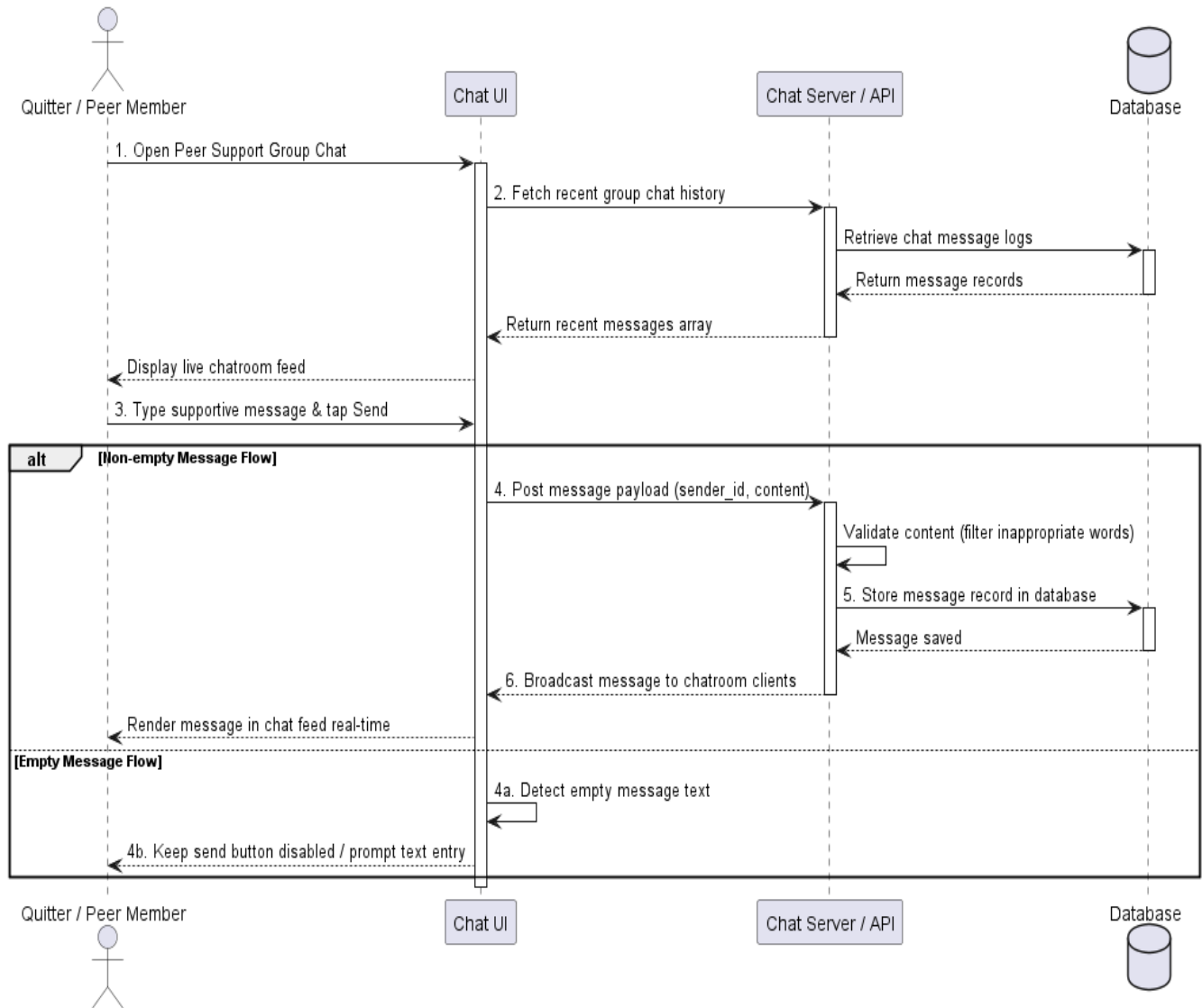
Figure 21: Sequence Diagram for Access Peer Support Group
