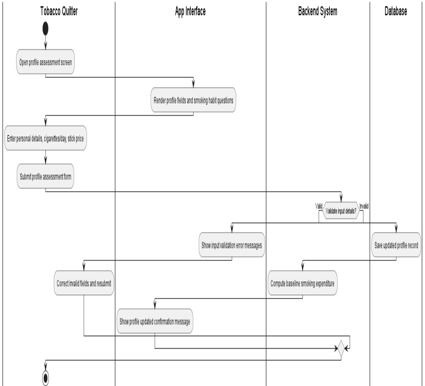
Figure 22: Swimlane Diagram for Manage Profile
