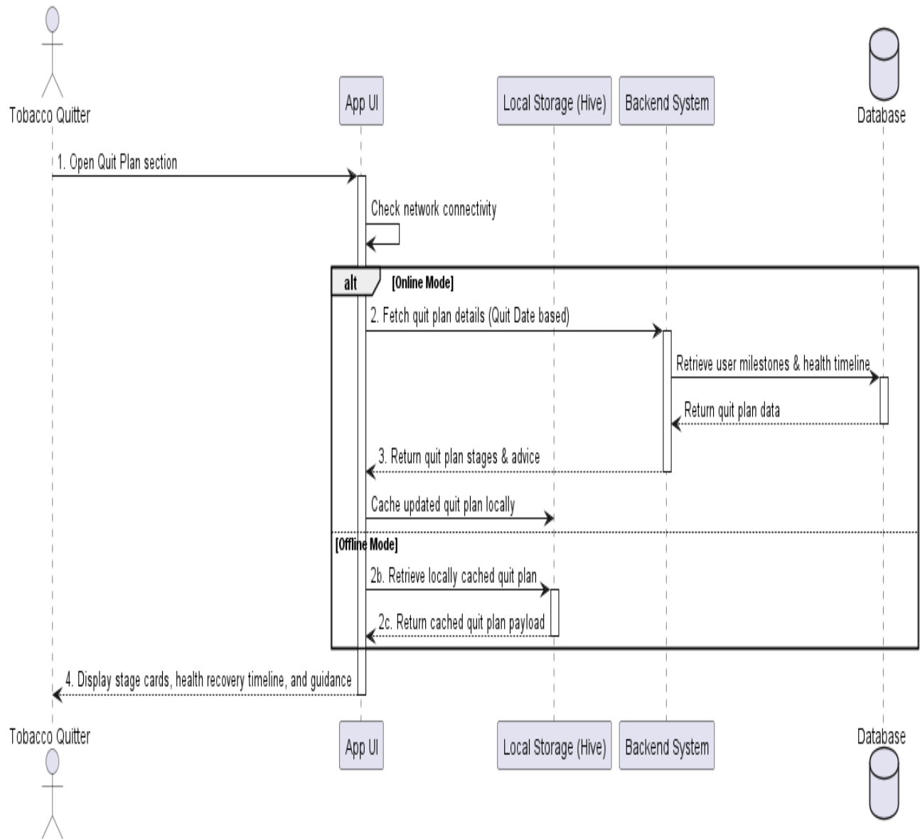
Figure 14: Sequence Diagram for View Quit Plan
