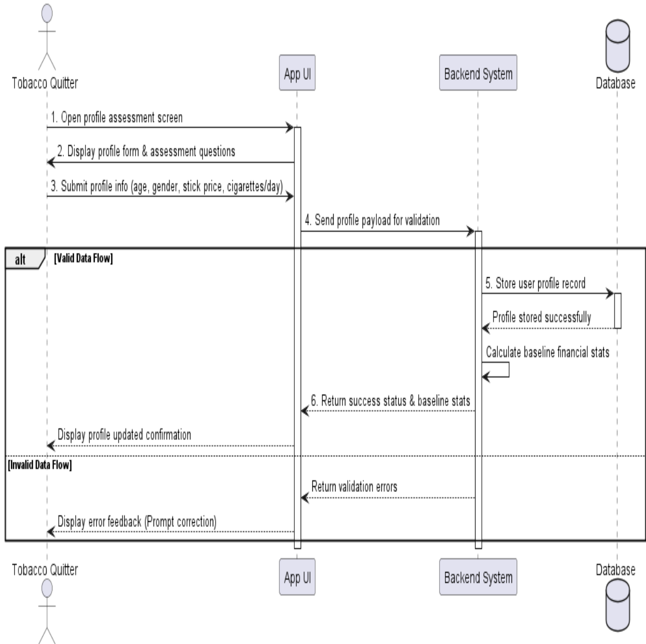
Figure 12: Sequence Diagram for Manage Profile
