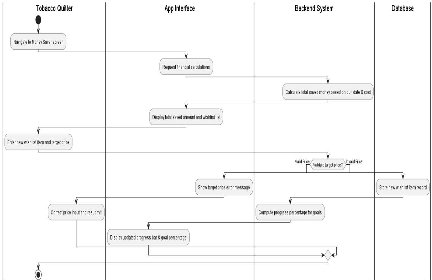
Figure 26: Swimlane Diagram for Track Saving
