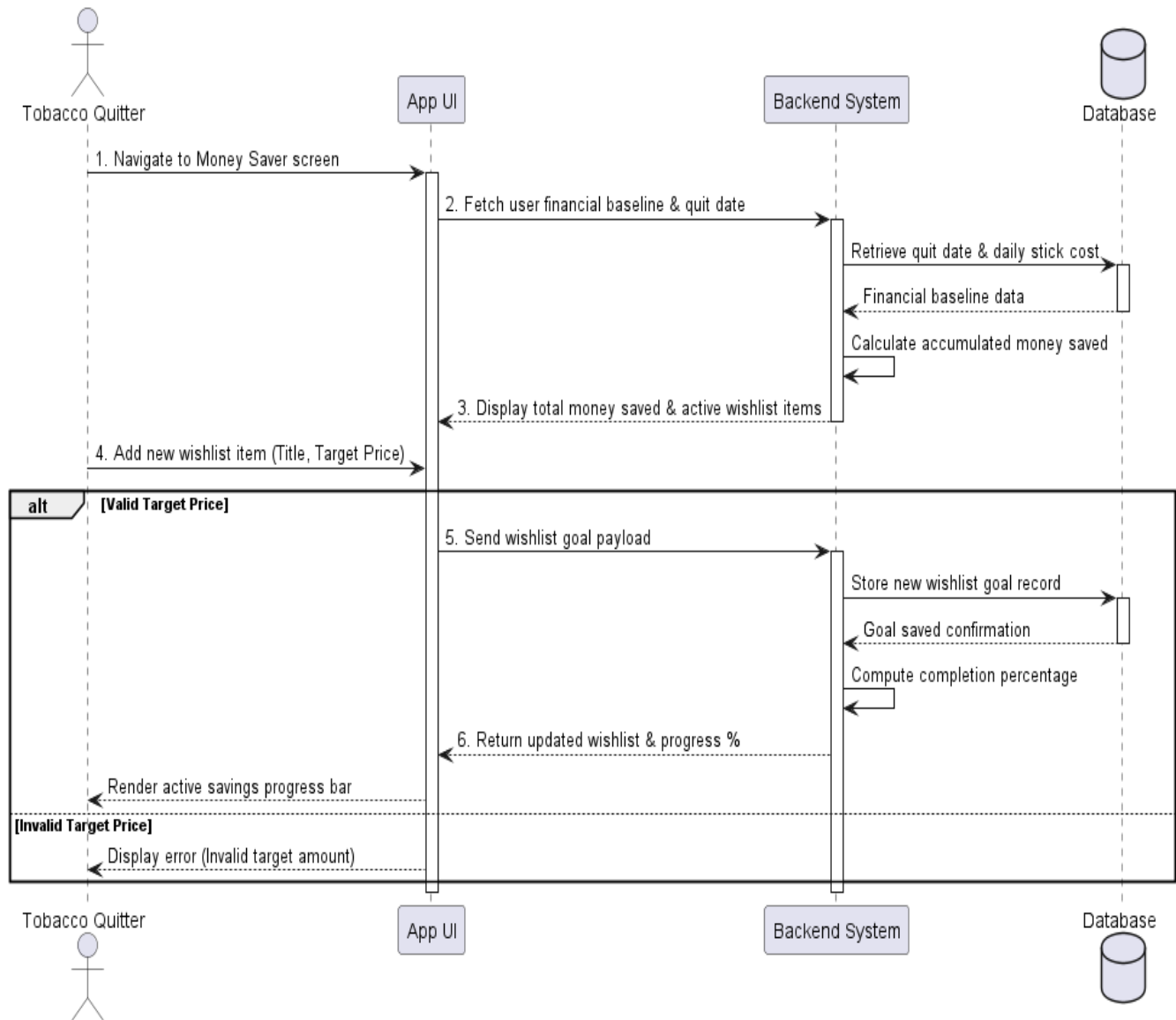
Figure 16: Sequence Diagram for Track Saving
