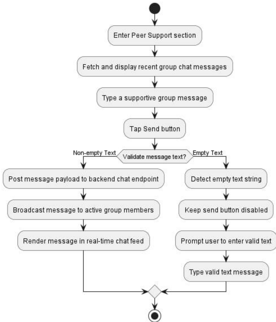
Figure 11: Activity Diagram for Access Peer Support Group
