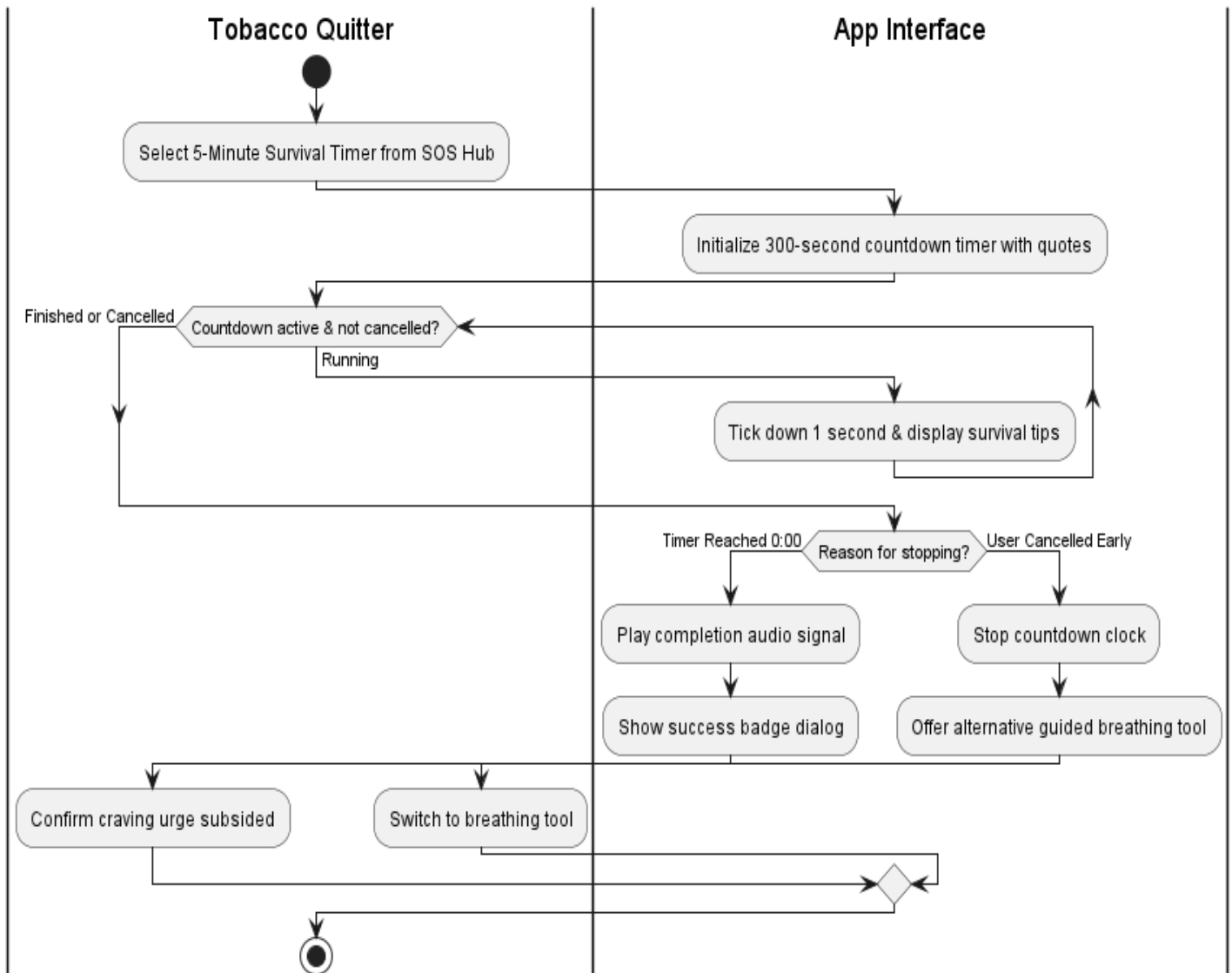
Figure 28: Swimlane Diagram for Start Survival Timer
